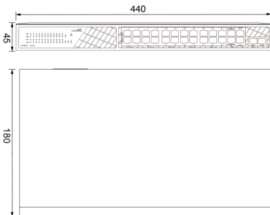
Dimension (mm)
